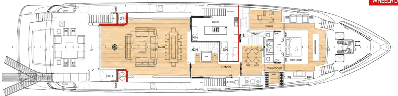
WHEELHOUSE DECK
