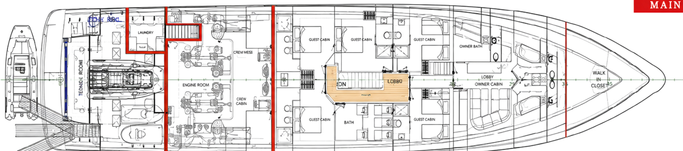
MAIN DECK
