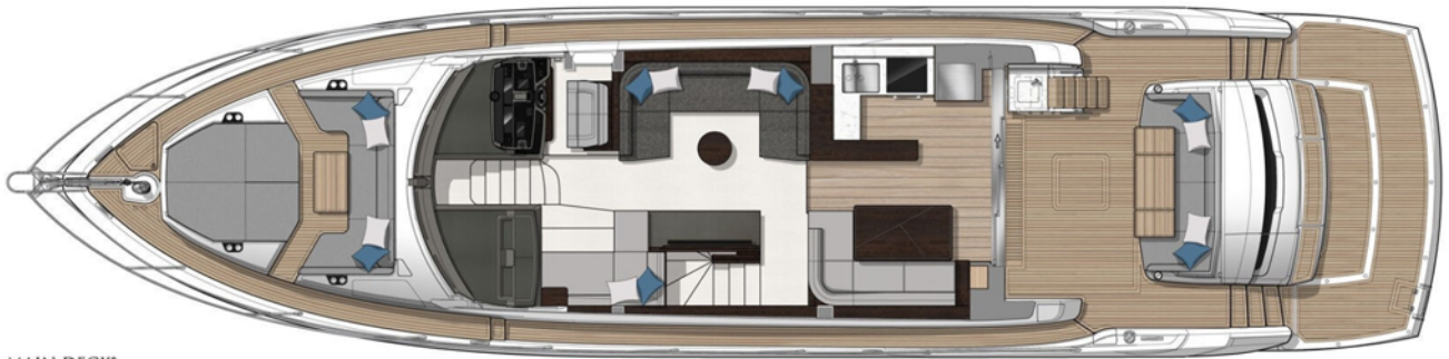
MAIN DECK*
